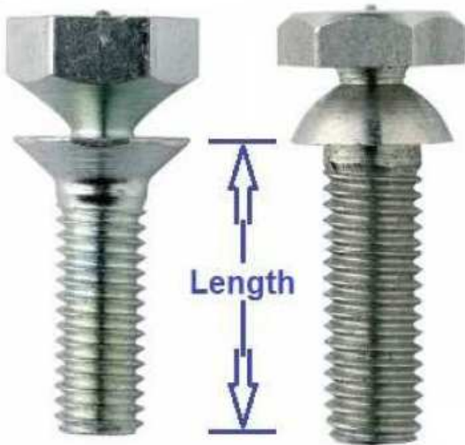
Flat head
