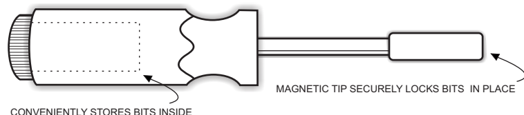
.250 HEX MAGNETIC SCREWDRIVER 8 INCH OVERALL LENGTH
