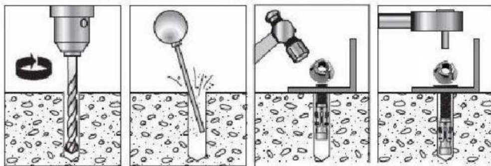
Install Socket
