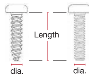
Tapping screw
